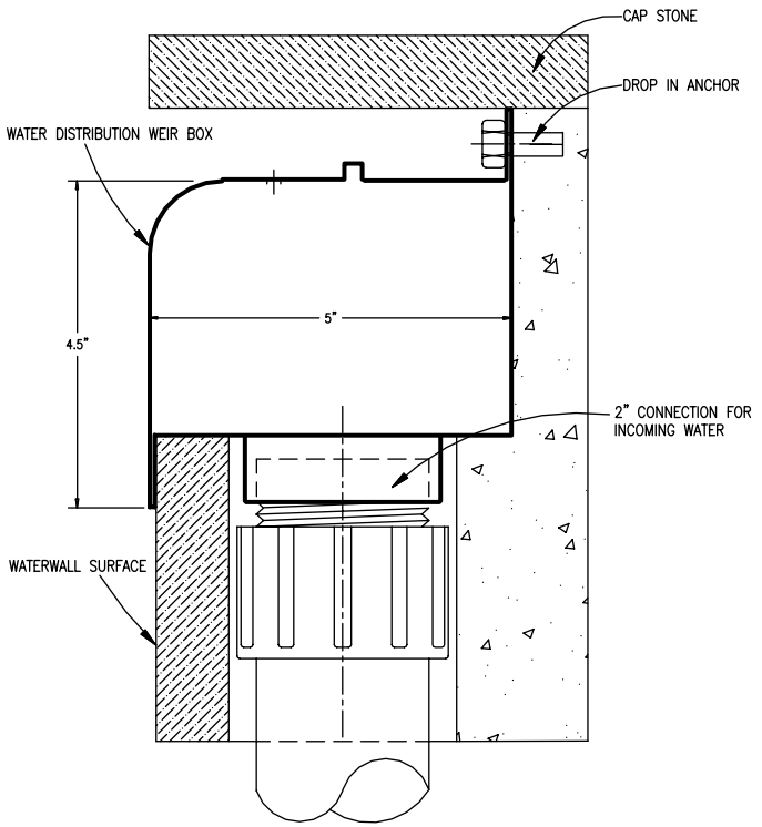
Accessories shown in drawing: 2" Male Adapter with 2" incoming water line by installer.
